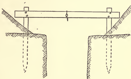
FIG. 6.—METHOD OF SETTING GRADE-PLANK.
